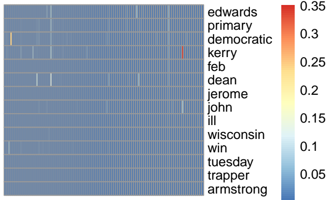
bg topic 83
