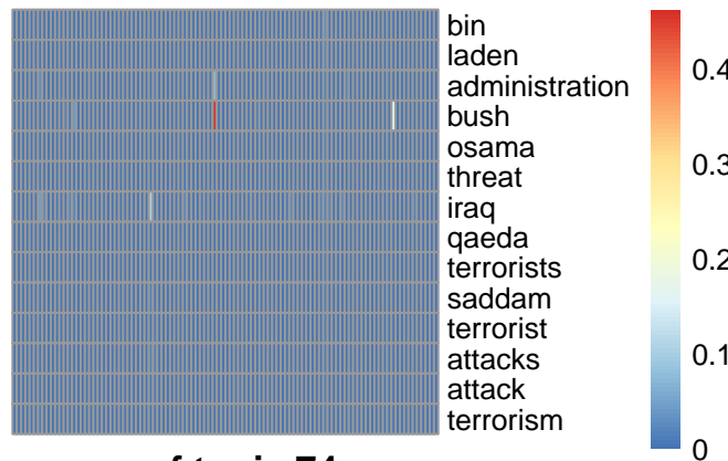
pmf topic 74
