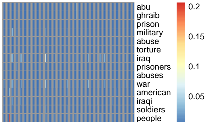
bg topic 57
