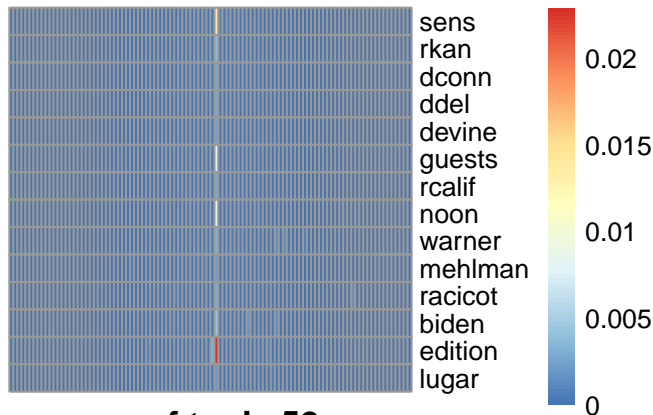
pmf topic 52
