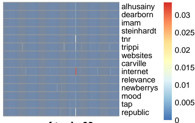
pmf topic 63
