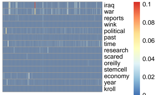
pmf topic 41
