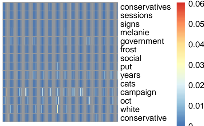
pmf topic 59
