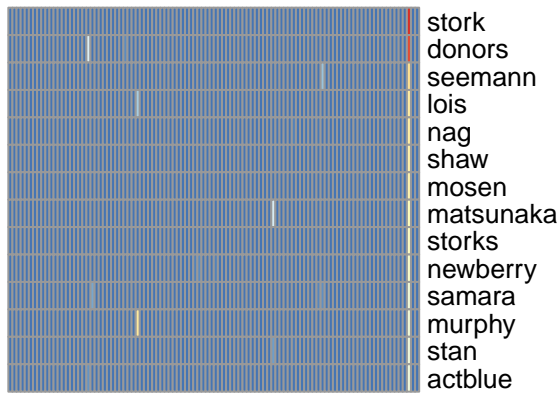
bg topic 98
