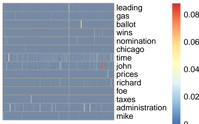
pmf topic 60
