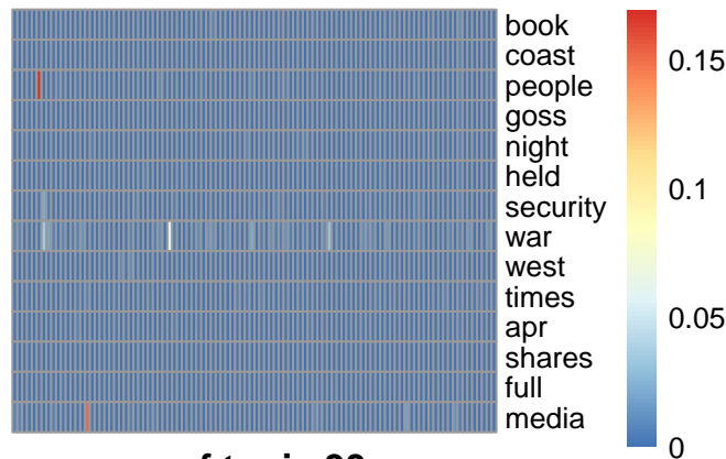
pmf topic 93
