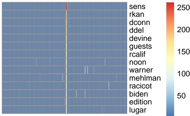
bg topic 52
