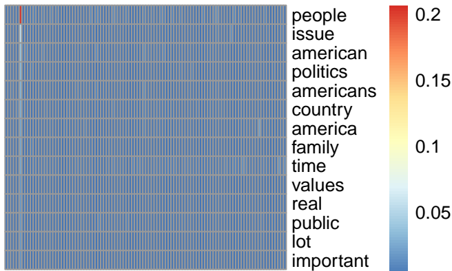
bg topic 6
