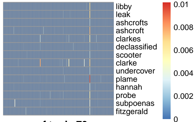
pmf topic 79
