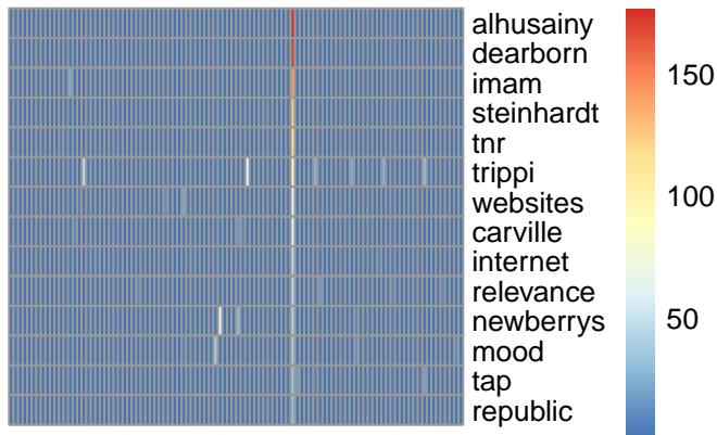
bg topic 63
