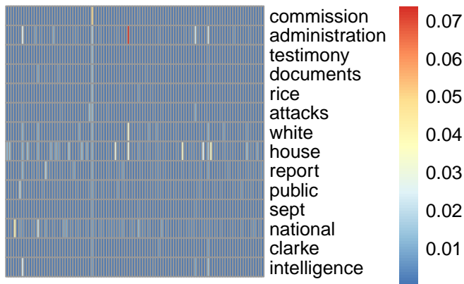
bg topic 34
