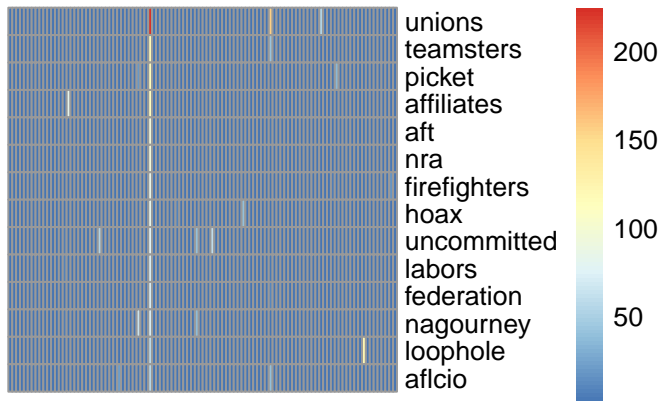
bg topic 37
