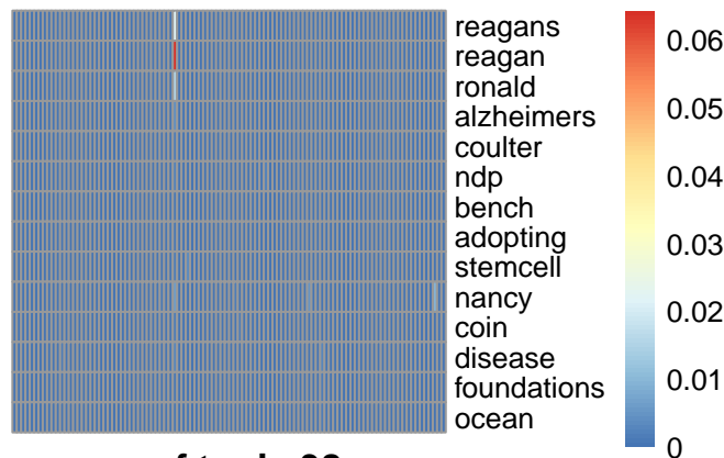
pmf topic 38
