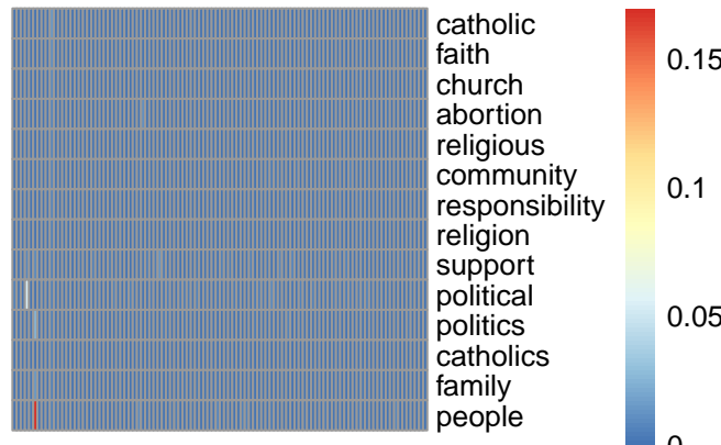
pmf topic 10
