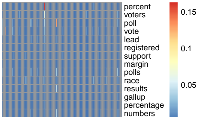
bg topic 36
