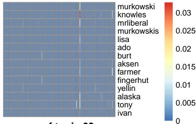
pmf topic 69
