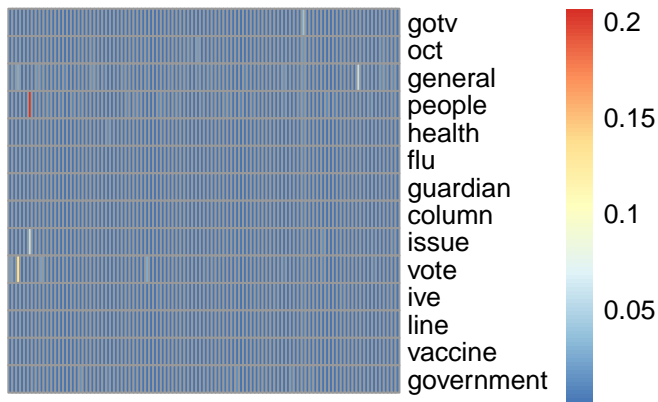
bg topic 76
