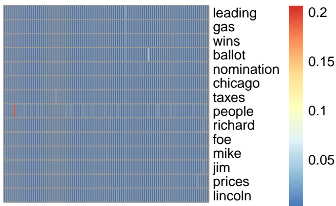
bg topic 60
