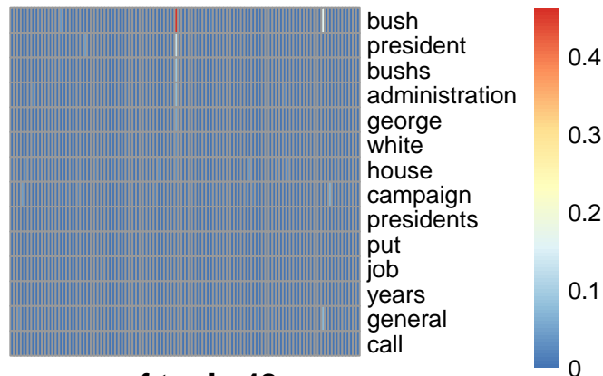
pmf topic 48
