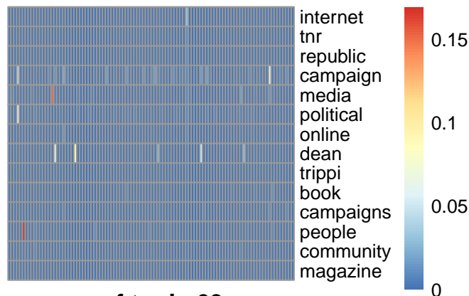
pmf topic 63
