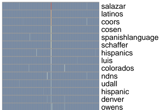
bg topic 51
