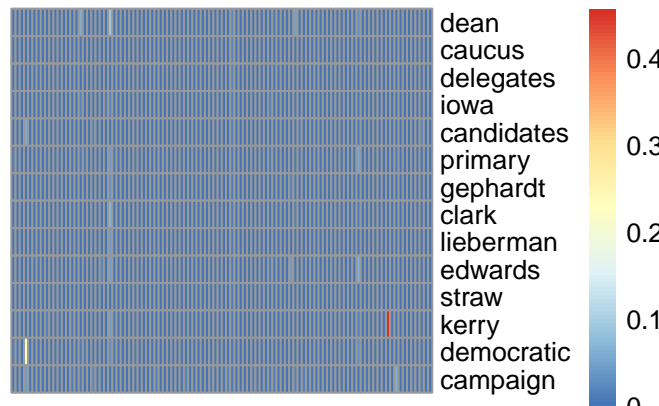
pmf topic 53
