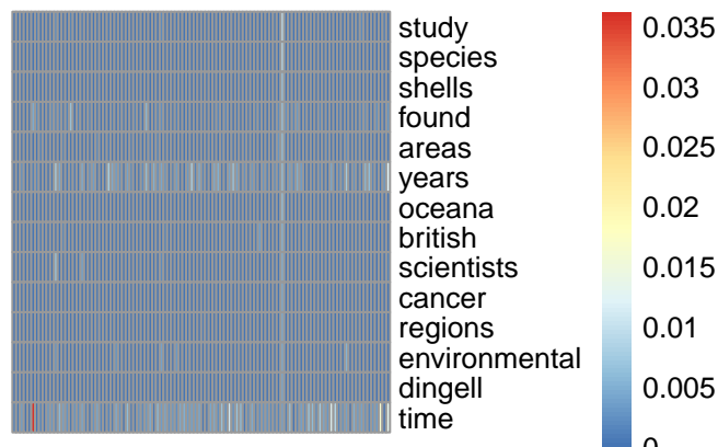
pmf topic 72
