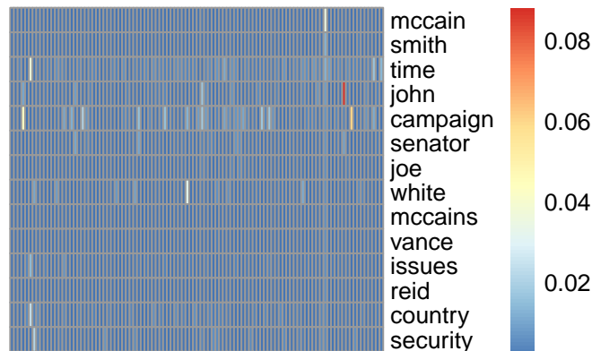
pmf topic 85
