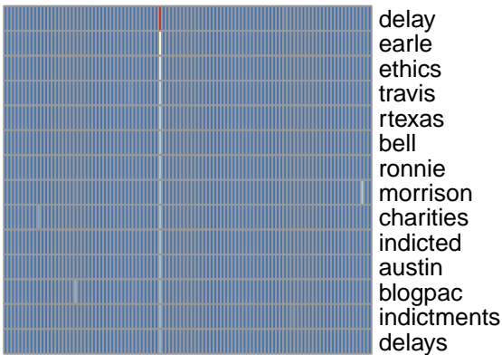
bg topic 43
