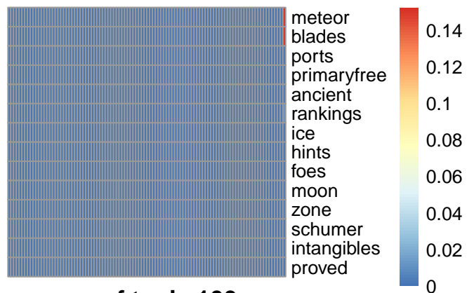
pmf topic 100
