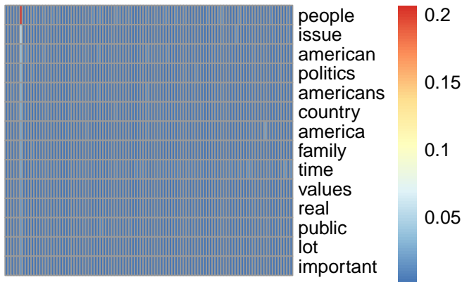
bg topic 6
