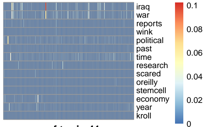
pmf topic 41
