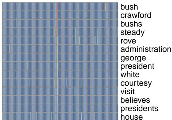
bg topic 48
