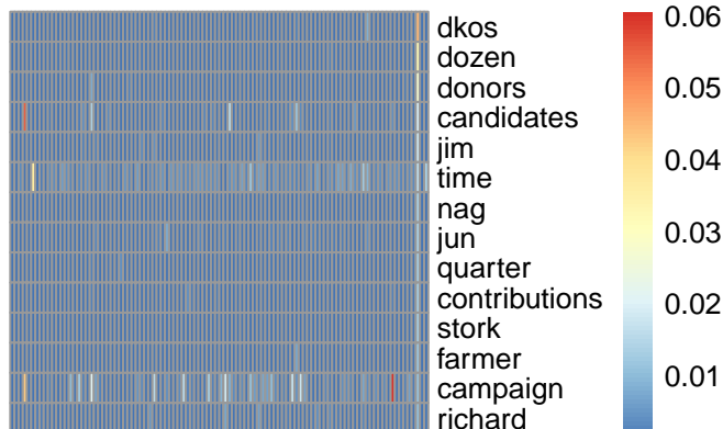
pmf topic 98
