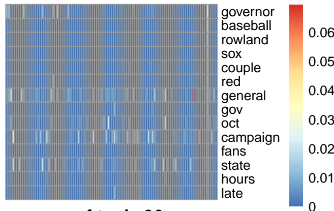
pmf topic 96
