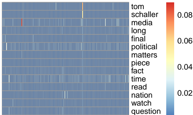
bg topic 64
