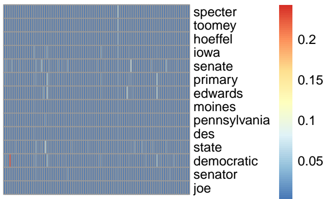
bg topic 62
