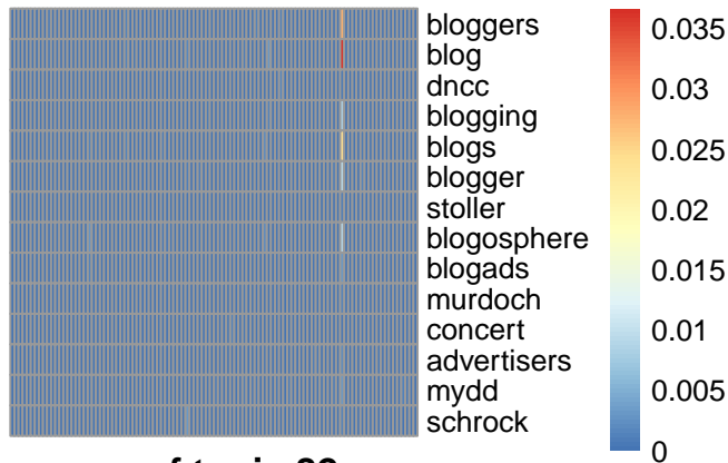
pmf topic 82
