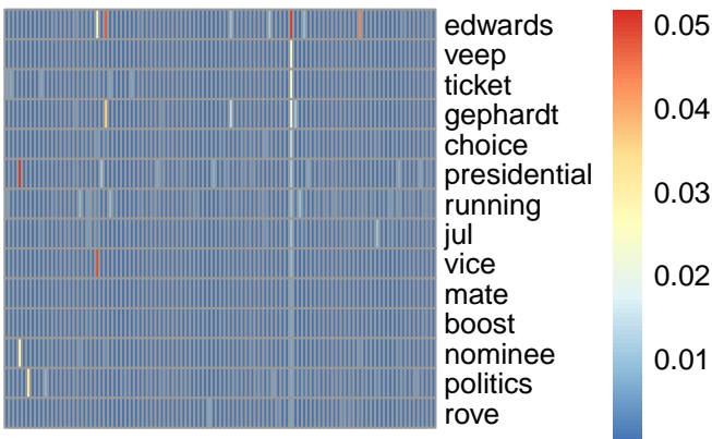
bg topic 67
