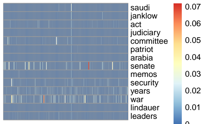
pmf topic 55
