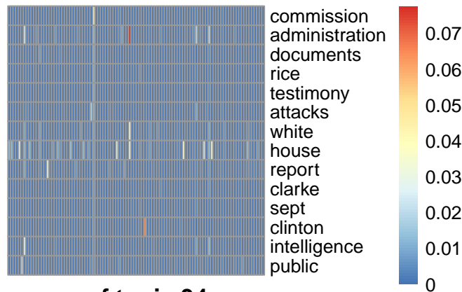
pmf topic 34
