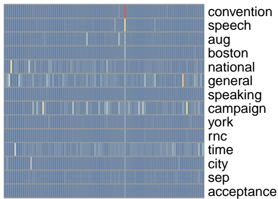
bg topic 61
