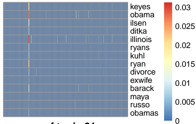
pmf topic 21
