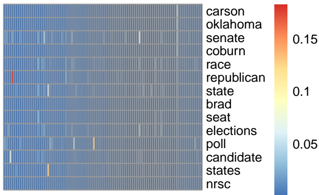
bg topic 88
