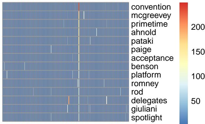
bg topic 61
