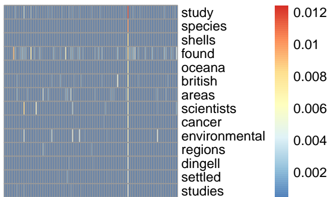
bg topic 72
