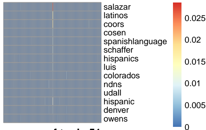
pmf topic 51
