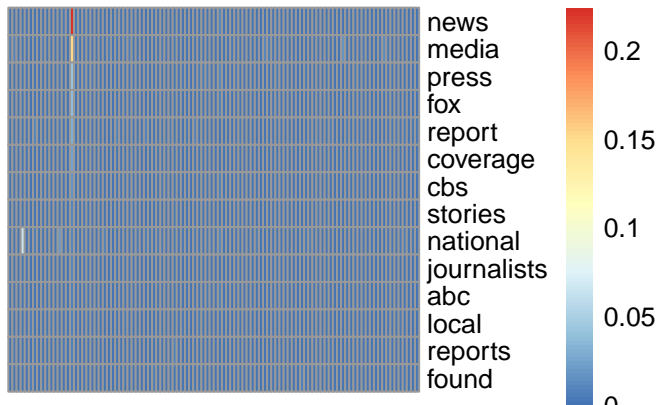
pmf topic 16
