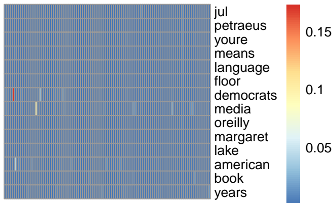
bg topic 87
