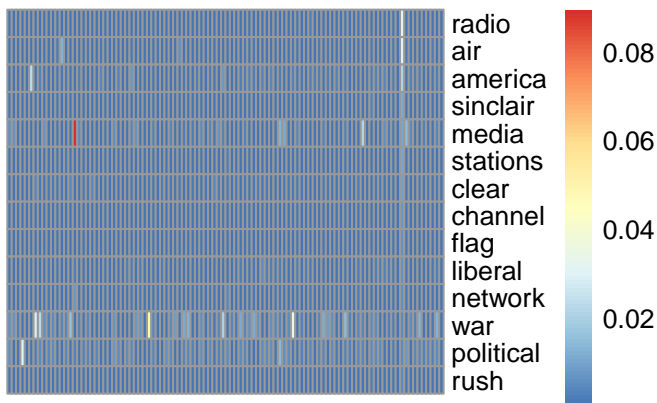
bg topic 91
