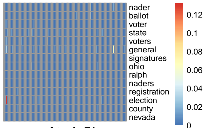
pmf topic 71
