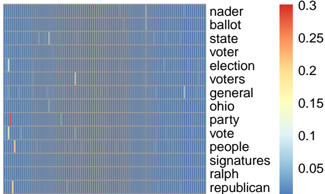
bg topic 71
