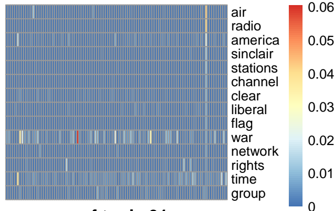
pmf topic 91
