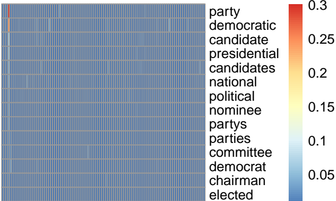
bg topic 4
