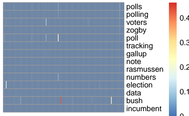
pmf topic 97
