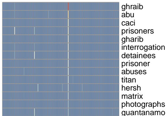
bg topic 57
