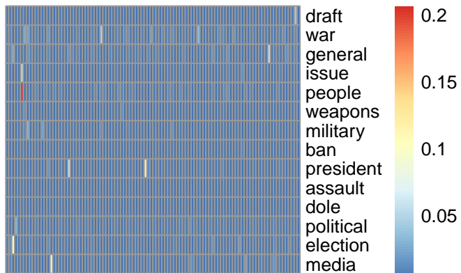
bg topic 99
