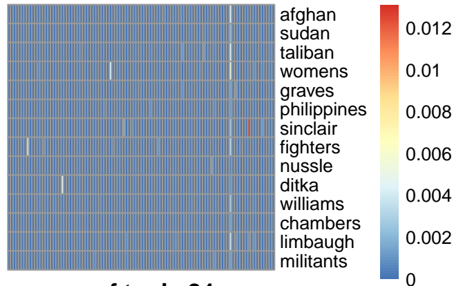
pmf topic 84
