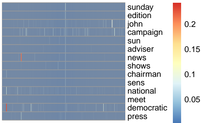
bg topic 52
