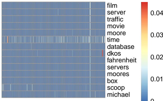
pmf topic 86
