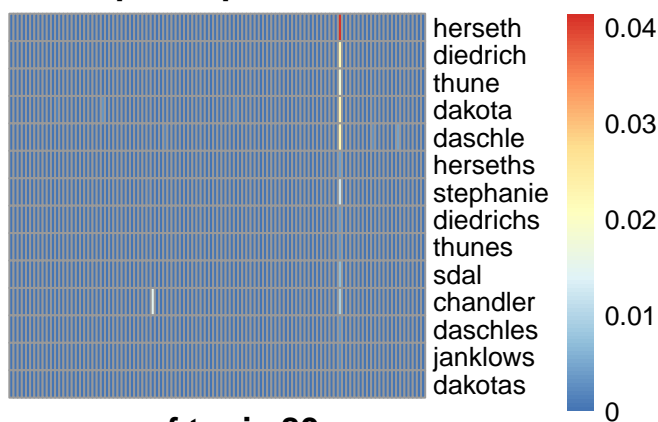
pmf topic 80
