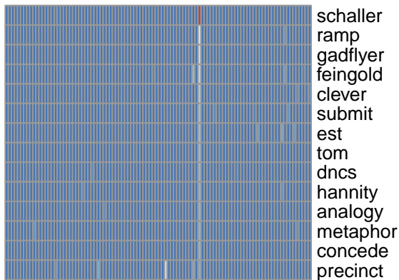
bg topic 64
