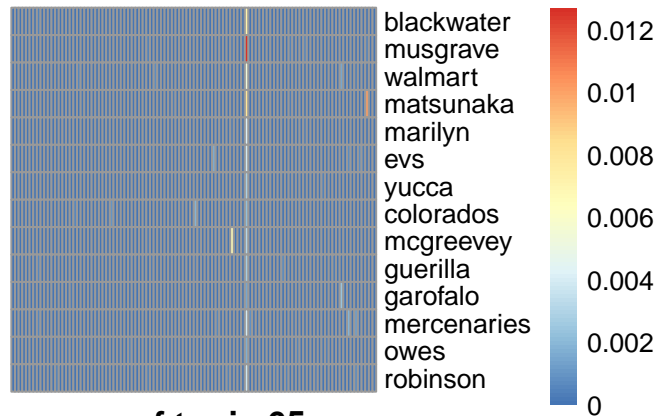
pmf topic 65
