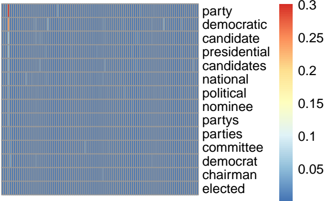
bg topic 4
