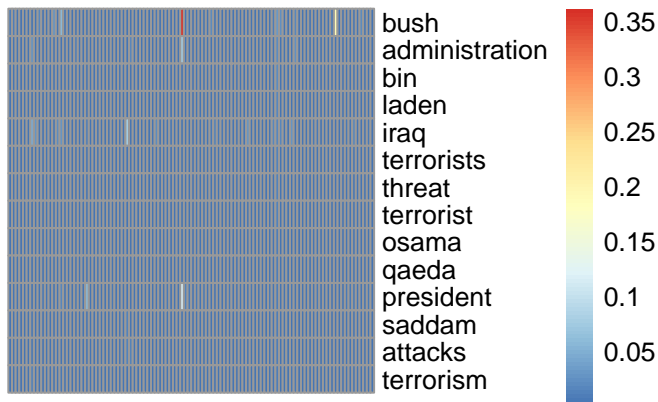
bg topic 74
