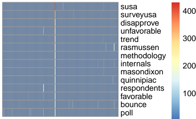
bg topic 46
