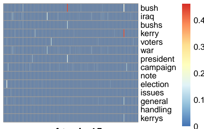
pmf topic 15
