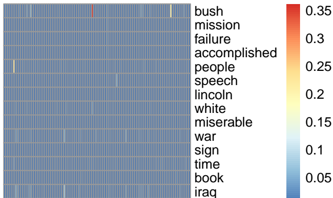
bg topic 56
