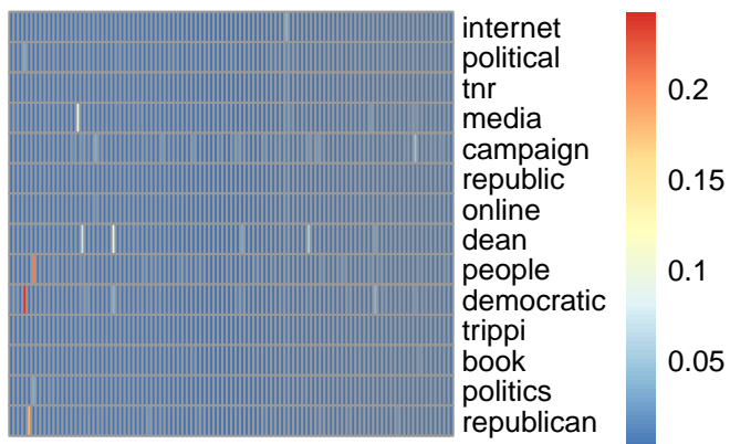
bg topic 63
