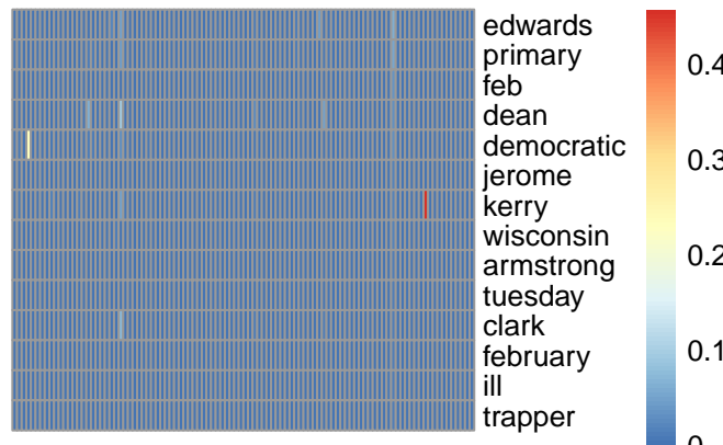
pmf topic 83
