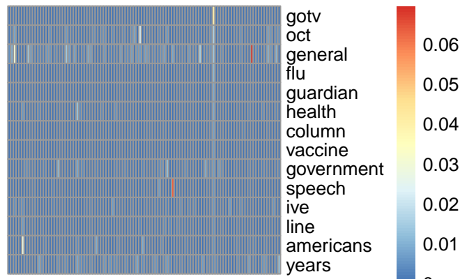
pmf topic 76
