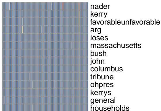
bg topic 90
