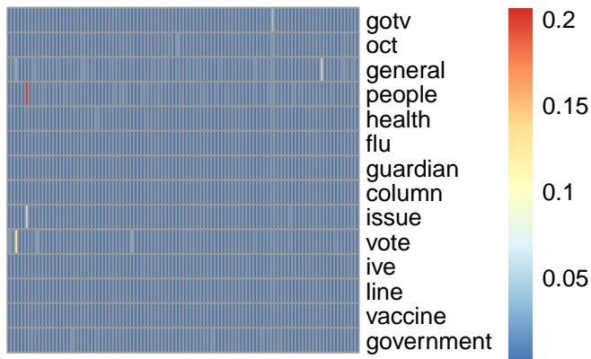
bg topic 76
