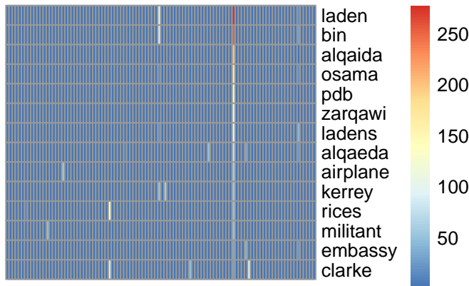
bg topic 74
