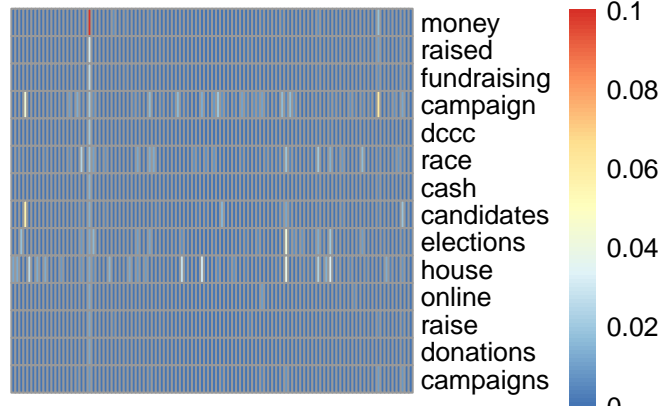
pmf topic 20
