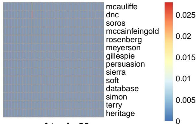
pmf topic 29
