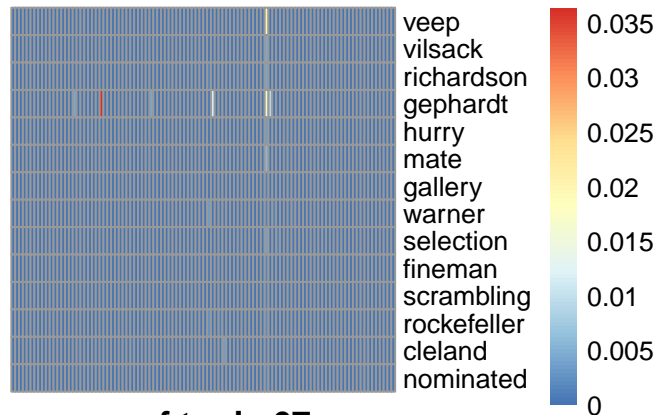
pmf topic 67
