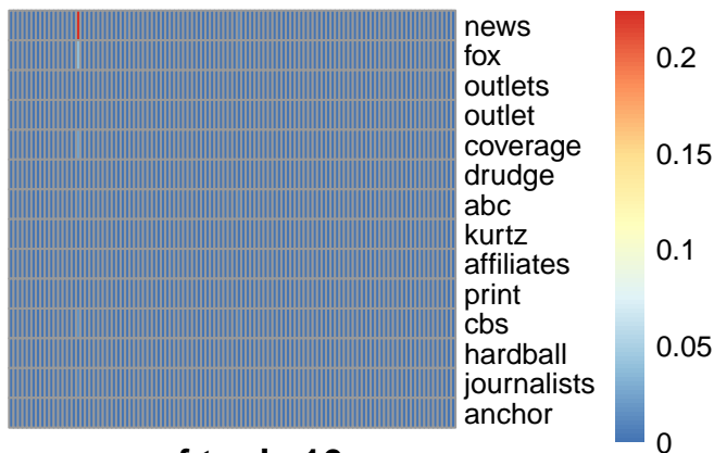
pmf topic 16
