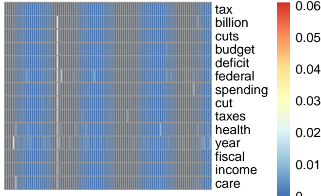
pmf topic 26
