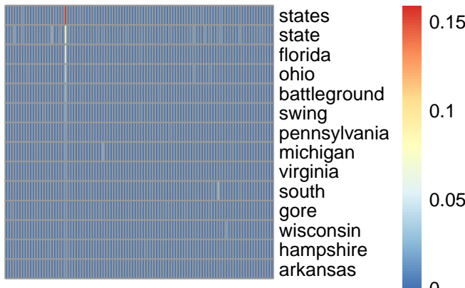
pmf topic 23
