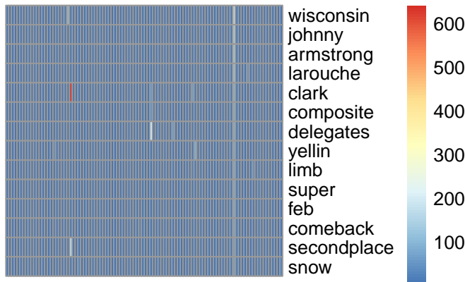
bg topic 83
