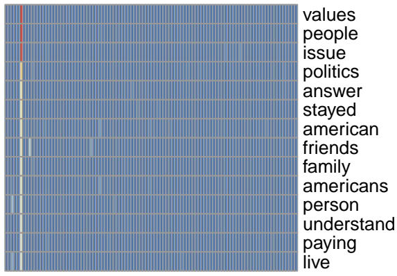
bg topic 6
