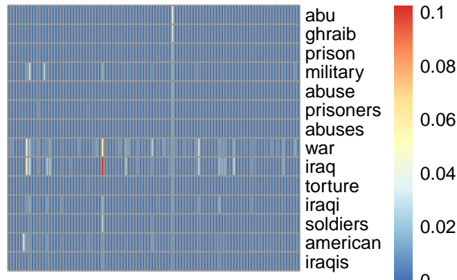
pmf topic 57
