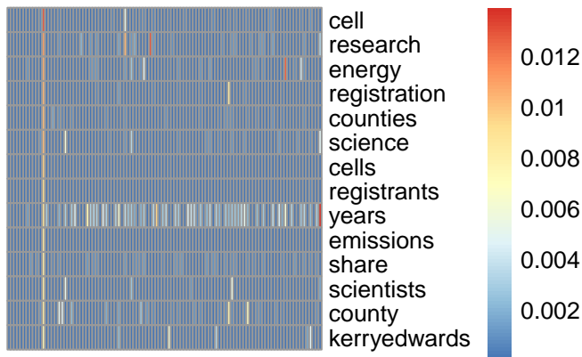
bg topic 12
