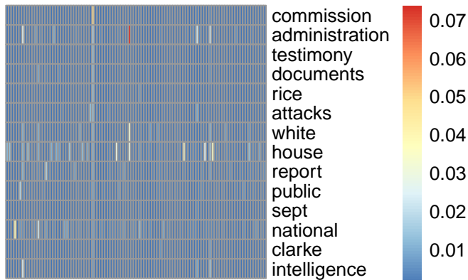
bg topic 34
