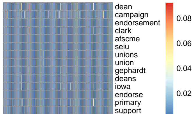
pmf topic 68
