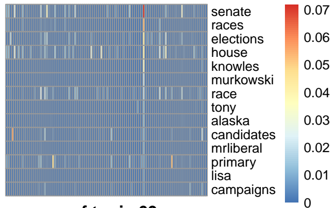
pmf topic 69
