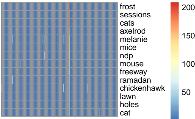
bg topic 59
