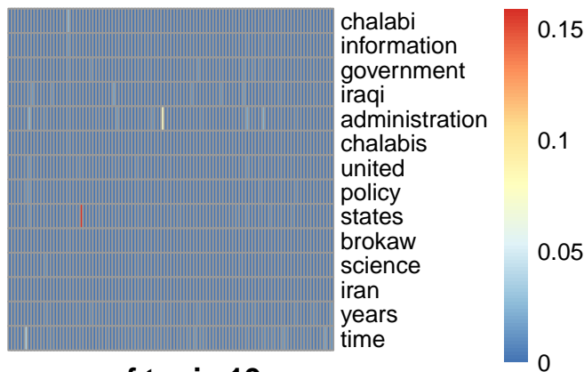
pmf topic 19
