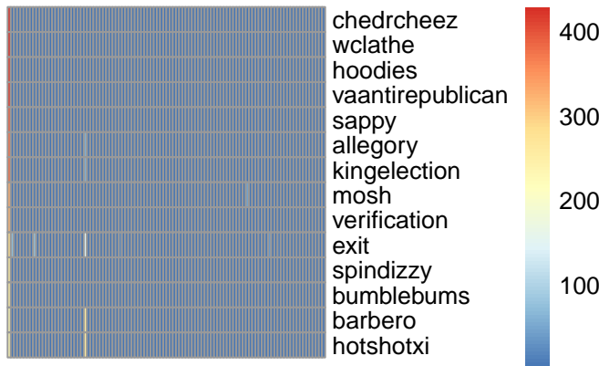
bg topic 1
