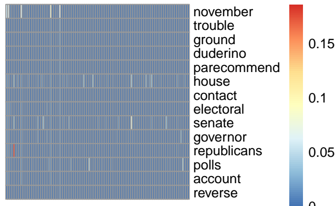
pmf topic 30
