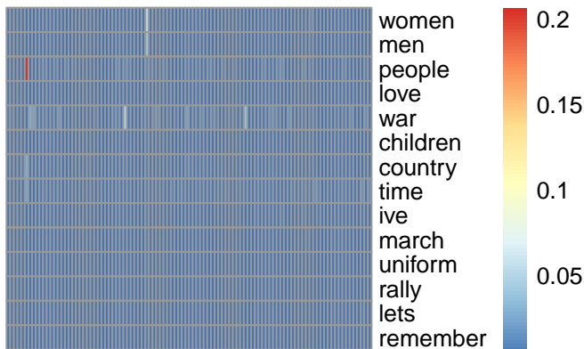
bg topic 39
